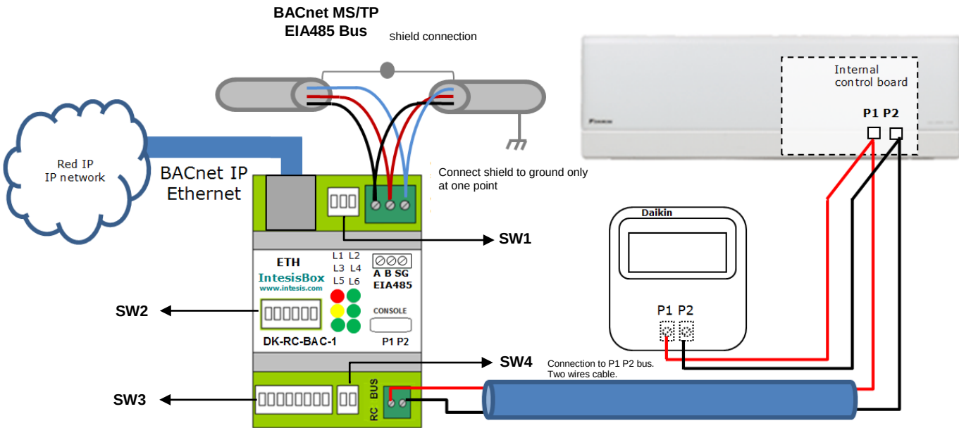
Connection diagram
