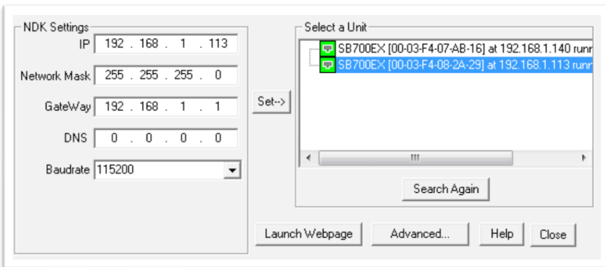
Figure 6.2-2 - IP Setup tool
