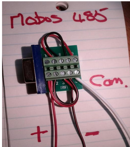
Figure 3.2-2 - Modbus RTU 485 Terminal Block
