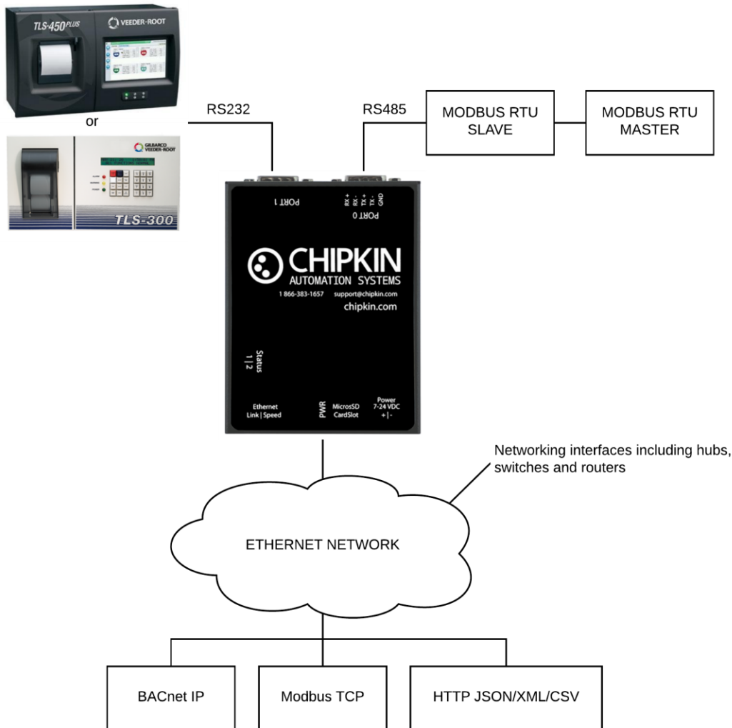
Figure 3.1-1 - Block Diagram
