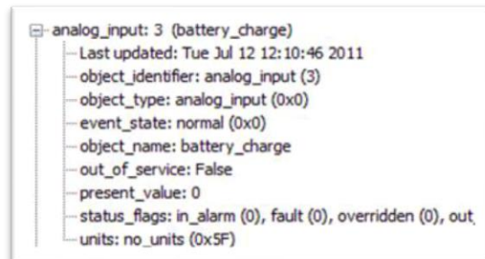
Figure 5.3-5 - CAS BACnet Explorer - Single Object
