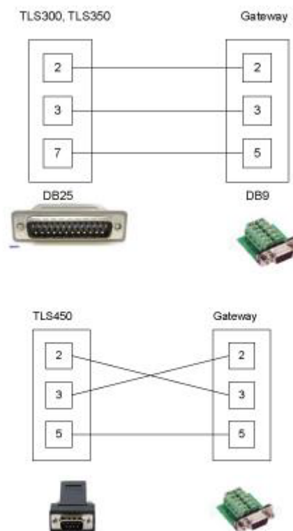
Figure 3.2-3 - RS232 Pin-out for Port 1 to the VeederRoot panel
