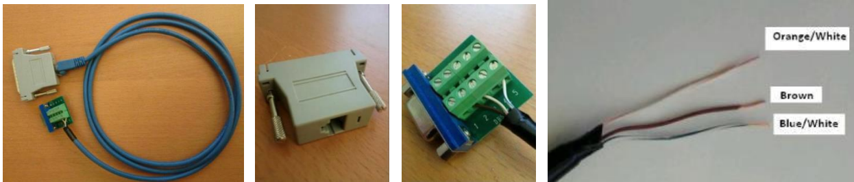
Figure 3.2-1 - Veeder Quick Assembly Cable for RS232
