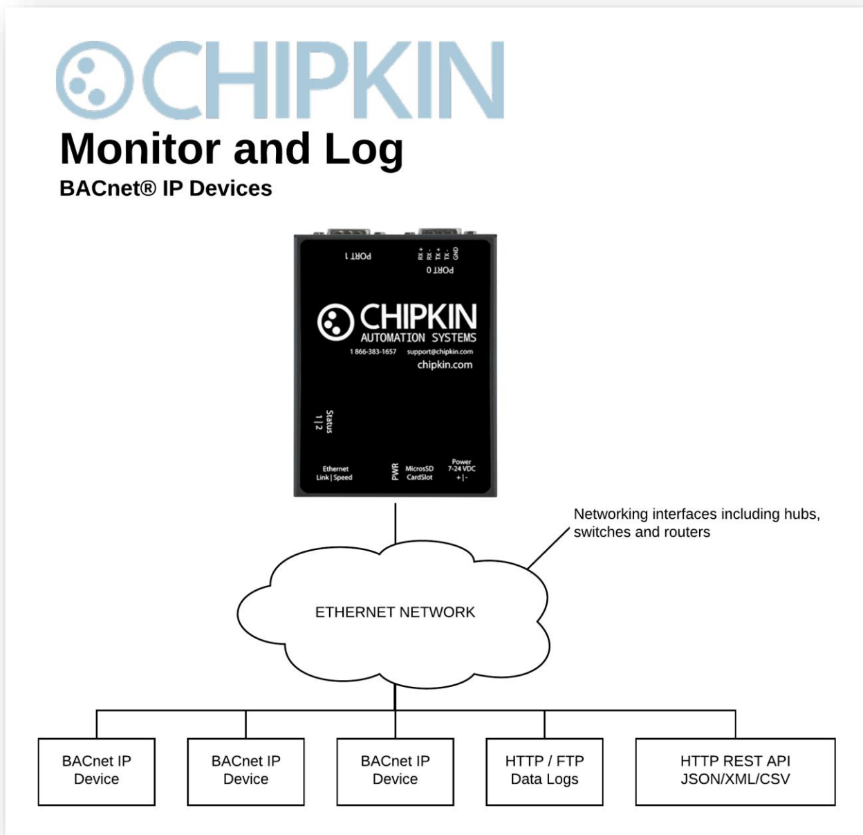
Figure 3.1-1 - Network Connections Block Diagram
