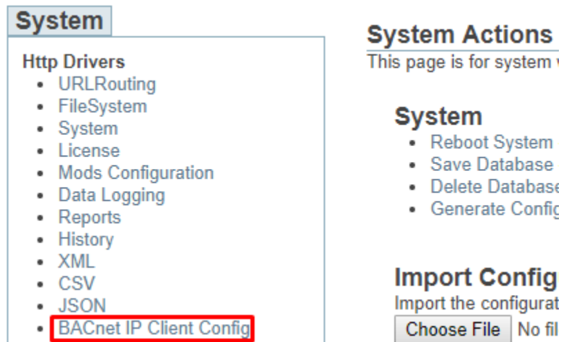
Figure 4.1-1 – BACnet IP Configuration Link
