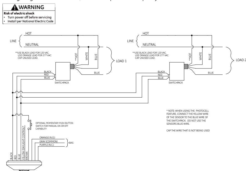
Wiring Diagram 3: One sensor, two switchpacks - occupancy control
