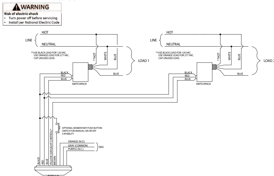
Wiring Diagram 3: One sensor, two switchpacks - occupancy control
