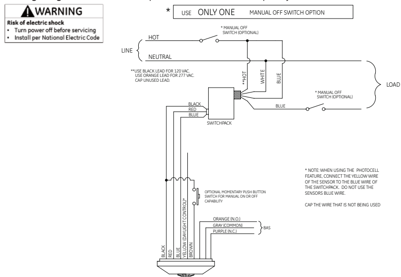
Wiring Diagram 2: One sensor, multiple switchpacks - one occupancy control, one daylight control
