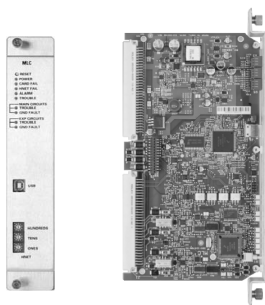
MLC → MXL Line Card [for FireFinder XLS]
